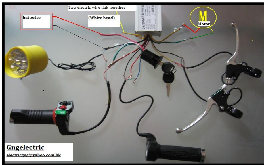
Electric wire installing
