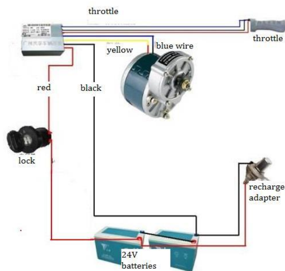
Electric wire installing
